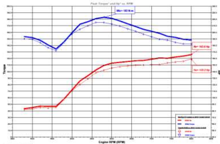
DYNOnote test "Team80 #1600 on 2016-11-24 @ 13:42:23" by Solex Auto, Inc
